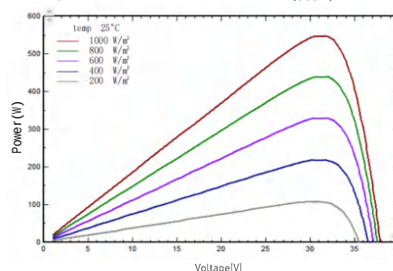
I-V/P-V Curve at Different Irradiation (565W)
