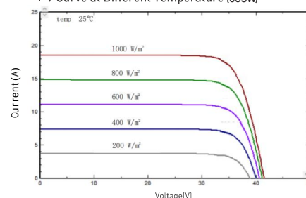
I-V/P-V Curve at Different Irradiation (605W)
