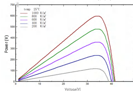
I-V/P-V Curve at Different Irradiation (625W)
