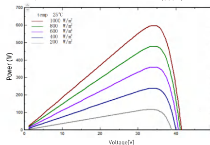
I-V/P-V Curve at Different Irradiation (630W)
