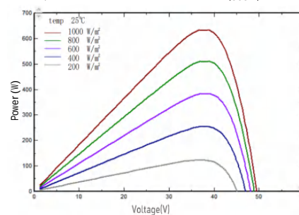
I-V/P-V Curve at Different Irradiation (660W)
