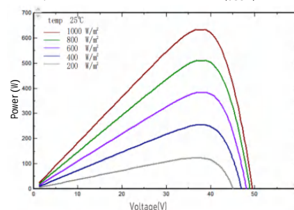
I-V/P-V Curve at Different Irradiation (685W)
