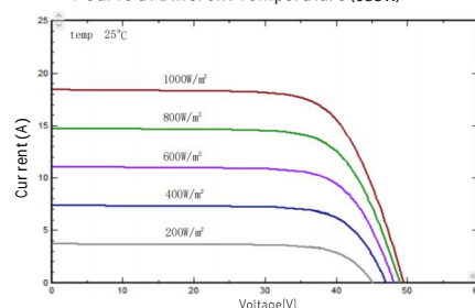
I-V/P-V Curve at Different Irradiation (685W)
