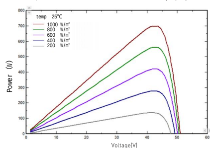
I-V/P-V Curve at Different Irradiation (715W)
