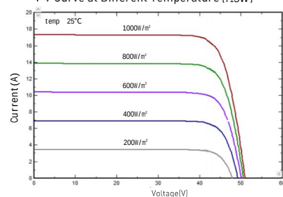
I-V/P-V Curve at Different Irradiation (715W)
