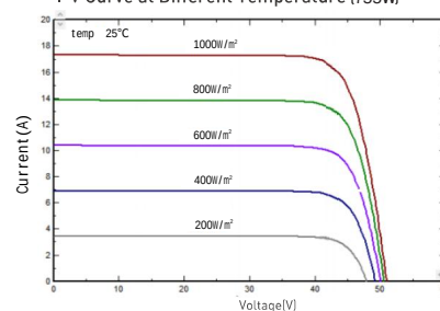
I-V/P-V Curve at Different Irradiation (755W)
