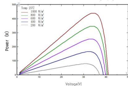
I-V/P-V Curve at Different Irradiation (420W)
