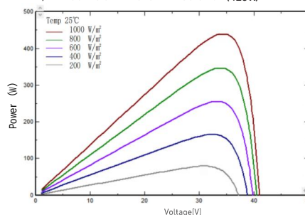
I-V/P-V Curve at Different Irradiation (420W)
