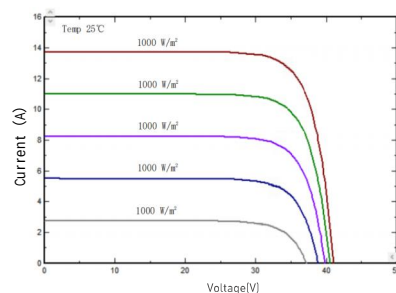
I-V/P-V Curve at Different Irradiation (440W)
