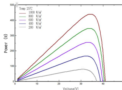
I-V/P-V Curve at Different Irradiation (440W)
