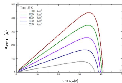
I-V/P-V Curve at Different Irradiation (445W)
