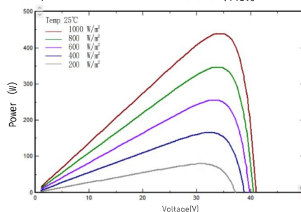
I-V/P-V Curve at Different Irradiation (445W)
