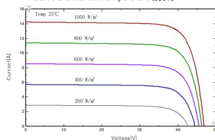
I-V/P-V Curve at Different Irradiation (530W)
