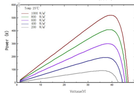
I-V/P-V Curve at Different Irradiation (530W)
