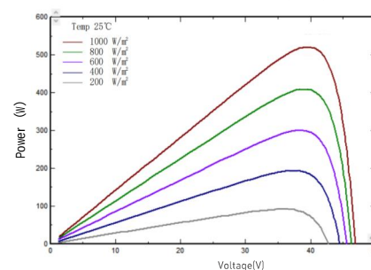
I-V/P-V Curve at Different Irradiation (530W)
