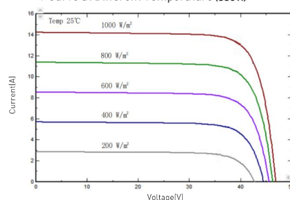
I-V/P-V Curve at Different Irradiation (530W)
