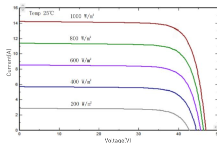
I-V/P-V Curve at Different Irradiation (550W)
