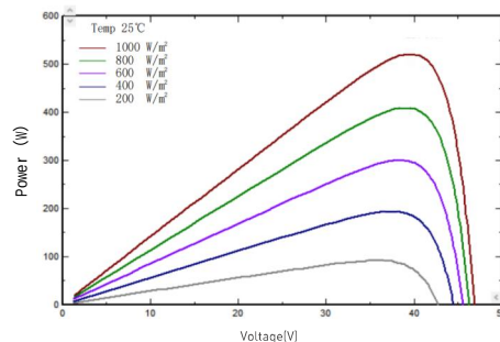
I-V/P-V Curve at Different Irradiation (550W)
