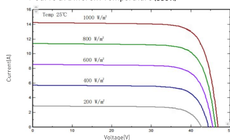
I-V/P-V Curve at Different Irradiation (550W)
