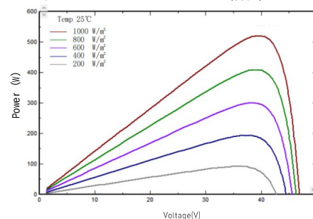
I-V/P-V Curve at Different Irradiation (555W)
