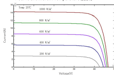
I-V/P-V Curve at Different Irradiation (555W)
