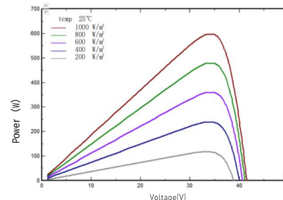
I-V/P-V Curve at Different Irradiation (605W)
