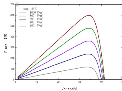
I-V/P-V Curve at Different Irradiation (605W)
