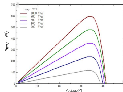
I-V/P-V Curve at Different Irradiation (610W)
