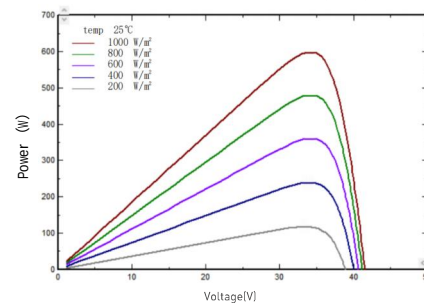
I-V/P-V Curve at Different Irradiation (610W)
