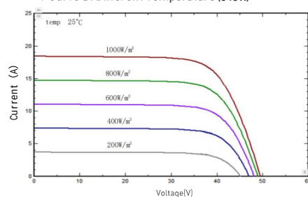
I-V/P-V Curve at Different Irradiation (640W)
