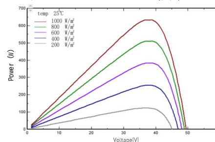
I-V/P-V Curve at Different Irradiation (640W)
