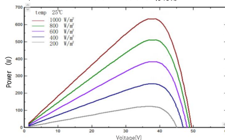
I-V/P-V Curve at Different Irradiation (640W)
