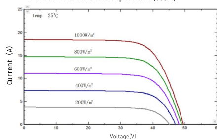
I-V/P-V Curve at Different Irradiation (665W)
