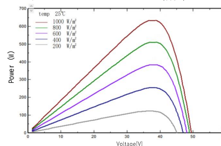
I-V/P-V Curve at Different Irradiation (665W)
