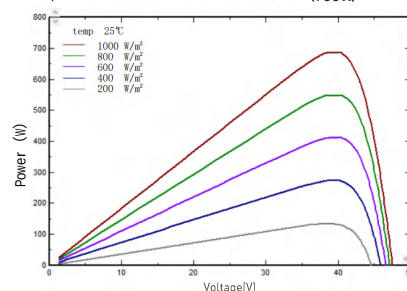
I-V/P-V Curve at Different Irradiation (700W)
