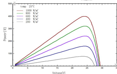
I-V/P-V Curve at Different Irradiation (410W)
