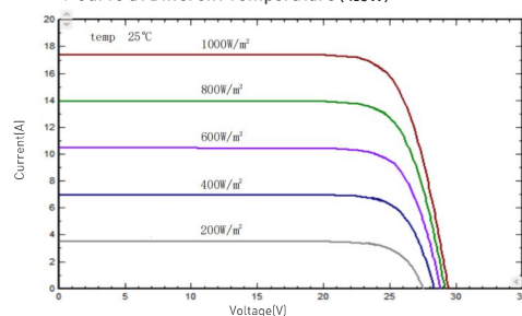
I-V/P-V Curve at Different Irradiation (410W)
