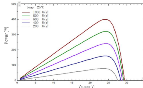
I-V/P-V Curve at Different Irradiation (415W)
