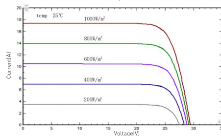
I-V/P-V Curve at Different Irradiation (415W)
