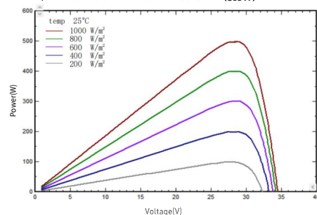
I-V/P-V Curve at Different Irradiation (510W)
