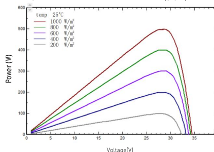
I-V/P-V Curve at Different Irradiation (510W)
