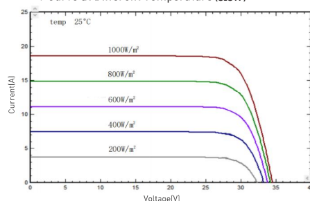
I-V/P-V Curve at Different Irradiation (515W)
