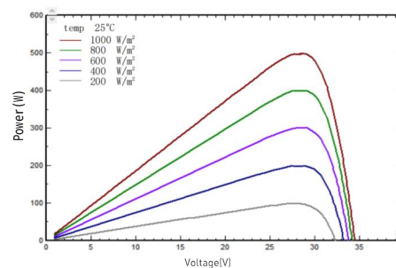
I-V/P-V Curve at Different Irradiation (515W)
