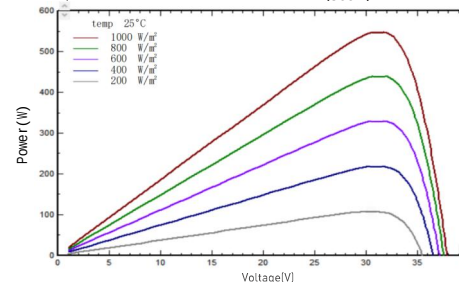
I-V/P-V Curve at Different Irradiation (560W)
