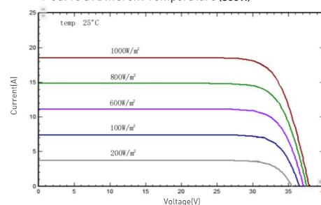
I-V/P-V Curve at Different Irradiation (560W)
