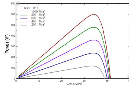
I-V/P-V Curve at Different Irradiation (615W)
