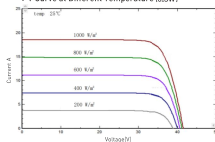
I-V/P-V Curve at Different Irradiance (615W)
