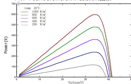
I-V/P-V Curve at Different Irradiance (615W)
