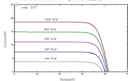
I-V/P-V Curve at Different Irradiation (620W)
