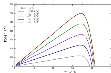
I-V/P-V Curve at Different Irradiation (620W)
