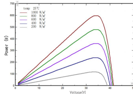
I-V/P-V Curve at Different Irradiation (620W)
