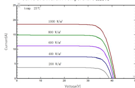
I-V/P-V Curve at Different Irradiation (620W)
