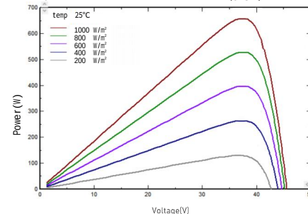
I-V/P-V Curve at Different Irradiation (675W)
