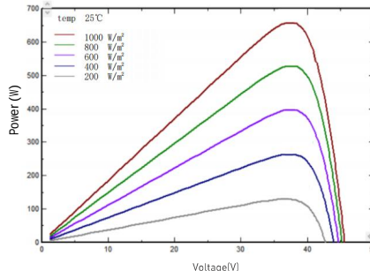
I-V/P-V Curve at Different Irradiation (675W)
