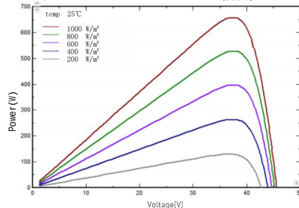
I-V/P-V Curve at Different Irradiation (680W)
