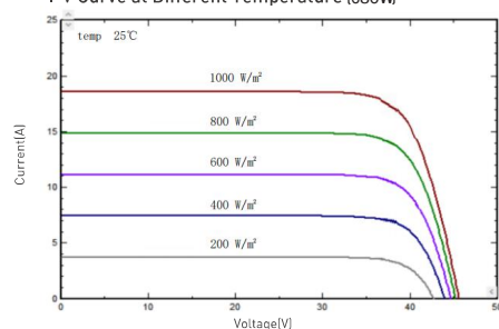
I-V/P-V Curve at Different Irradiation (680W)
