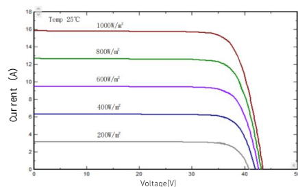
I-V/P-V Curve at Different Irradiation (450W)
