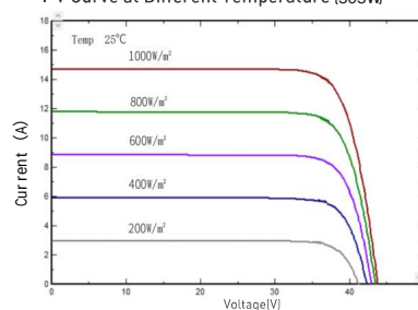
I-V/P-V Curve at Different Irradiation (505W)
