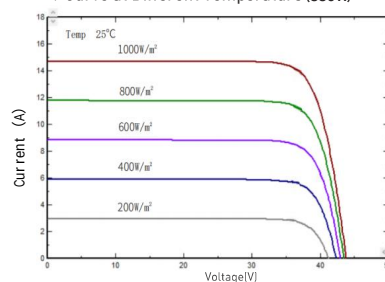
I-V/P-V Curve at Different Irradiation (530W)
