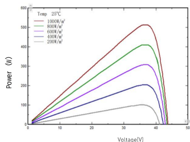
I-V/P-V Curve at Different Irradiation (530W)
