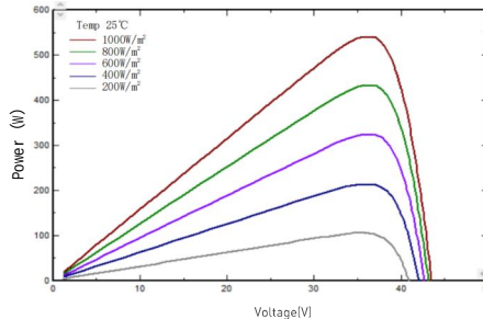
I-V/P-V Curve at Different Irradiation (565W)
