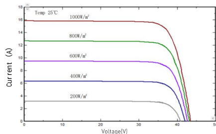
I-V/P-V Curve at Different Irradiation (565W)
