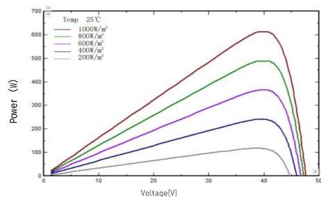
I-V/P-V Curve at Different Irradiation (620W)
