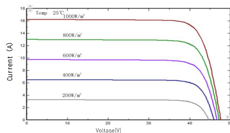
I-V/P-V Curve at Different Irradiation (620W)
