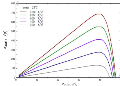
I-V/P-V Curve at Different Irradiation (730W)
